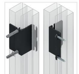
Concealed fastening brackets
