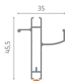
Handlebar
